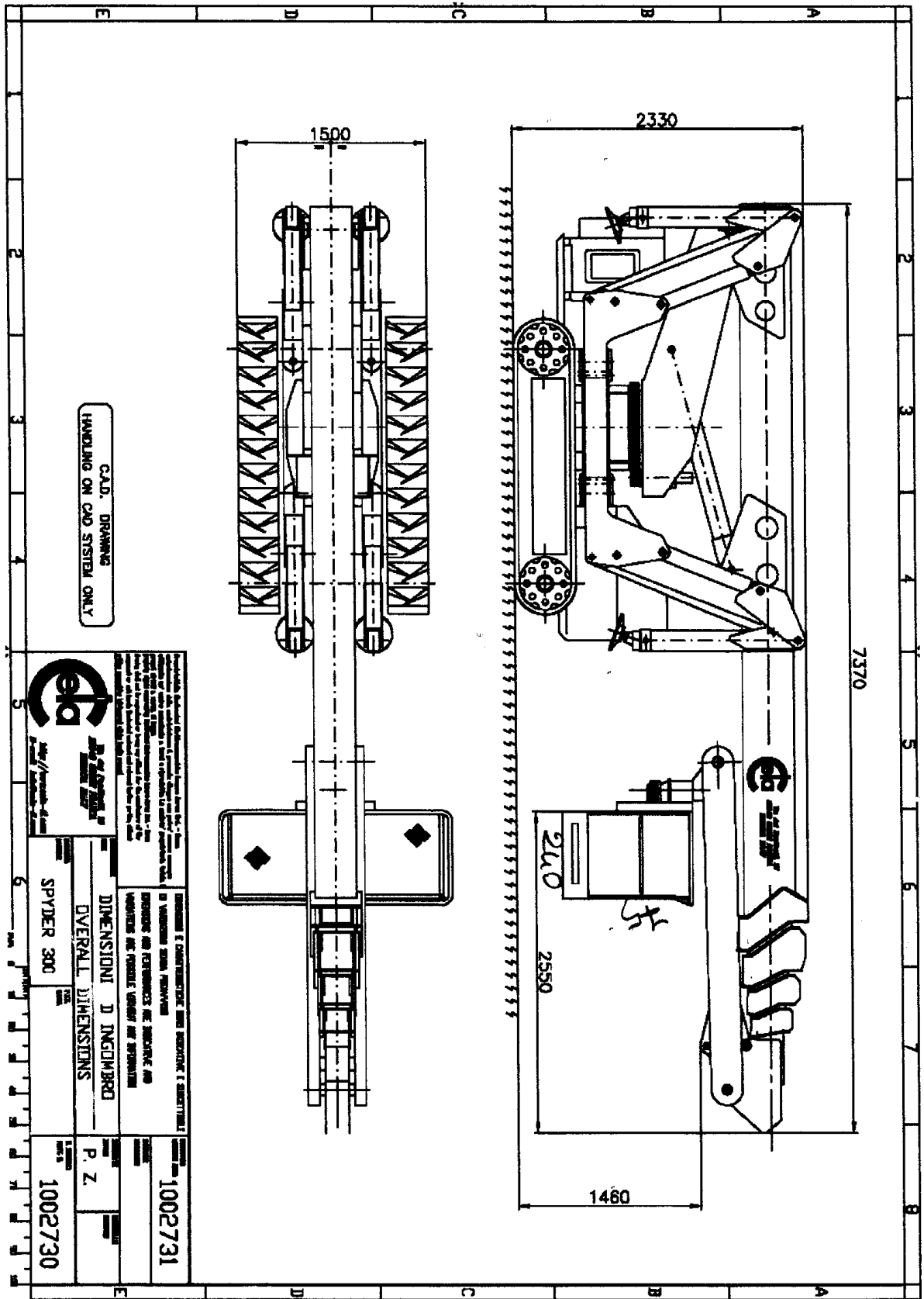
DWG. 1002730
